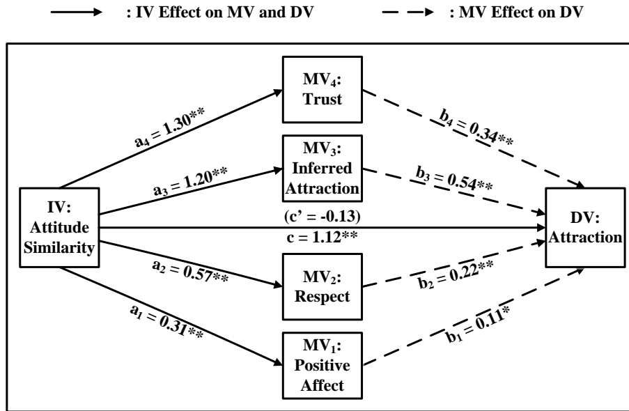
Figure 3. Results from a four-MV parallel model analysis of Experiment 3. The IV effects on all the four MVs ( a_1 , a_2 , a_3 , and a_4 ) are independent of each other. As in the previous figures, the c coefficient represents the zero-order relation between the IV and DV, whereas the c' path coefficient represents the relation between the IV and DV controlling for the four mediating variables. * p = .05 ; ** p < .01 .
